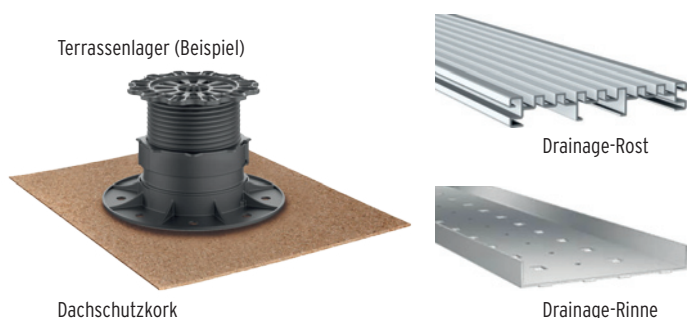
Drainage-Rinne
