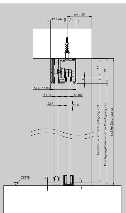
PLANEO 120, DECKENMONTAGE FÜR GLASANLAGEN CEILING MOUNTING FOR GLASS DOOR SYSTEM
