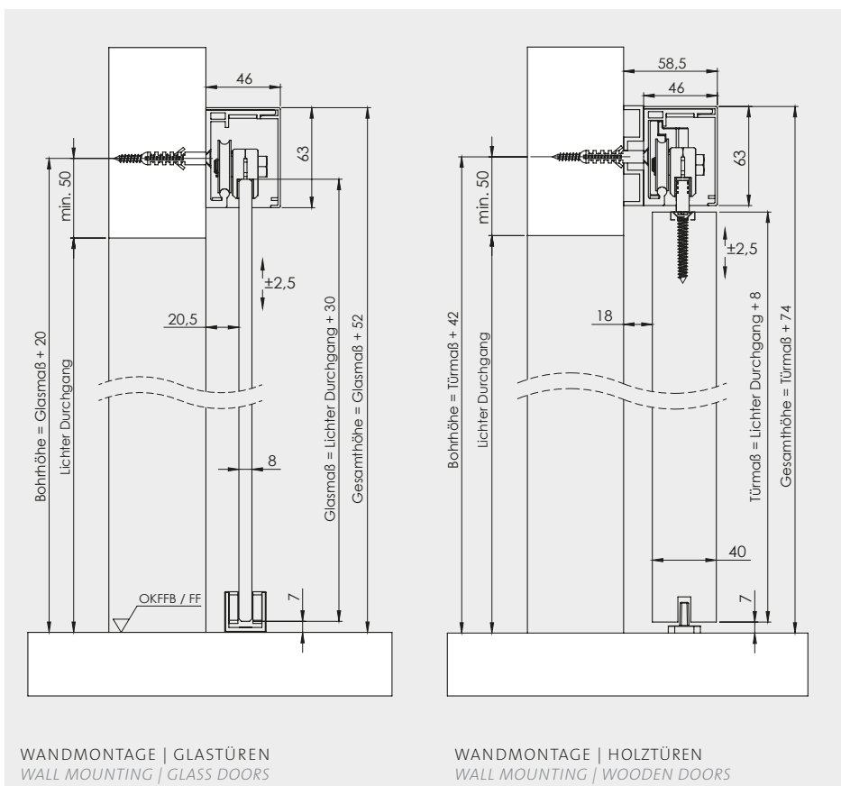
PLANE0 60 PRO WANDMONTAGE WALL MOUNTING
